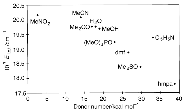
Fig. 9 A plot of the i.c.t. energy ( E_{\text{i.c.t.}} ) vs. the solvent Gutmann donor number for salt 2
