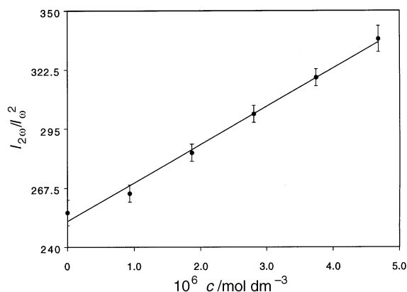
Fig. 3 Ratio of the intensities I_{200}/I_0^2 vs. the molar concentration; experimental data and linear fit for salt 2 in acetonitrile. Each point is the average of four separate measurements and error bars show the standard deviations
