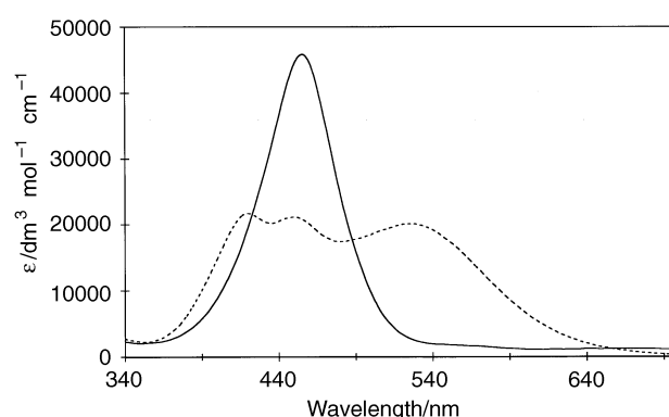
Fig. 8 The UV/VIS spectra of salt 4 in hmpa (—) and in dmf (---)
