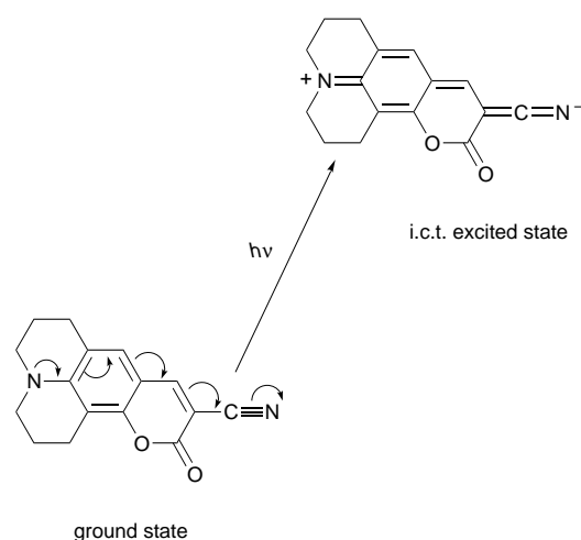
Fig. 5 Simplified representation of the formation of one possible i.c.t. excited state of C-523
